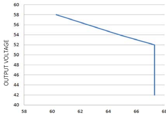
Figure 4. 54V DC output: Power limit, Current limit and shutdown profile at V_{IN} = 185V_{AC} .
