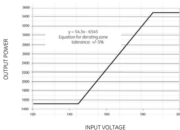
Figure 17. Output power derating below V_{IN} of 185V AC
